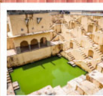
♡▽ Panna Meena
