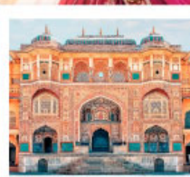
♡♡▽ Amber Fort
